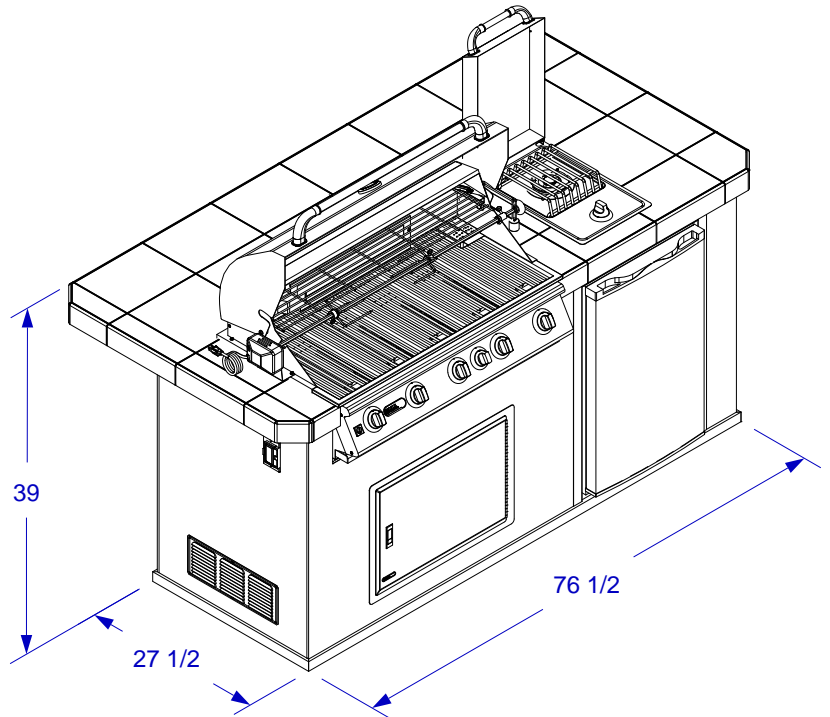
ISOMETRIC VIEW
