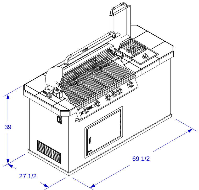
ISOMETRIC VIEW
