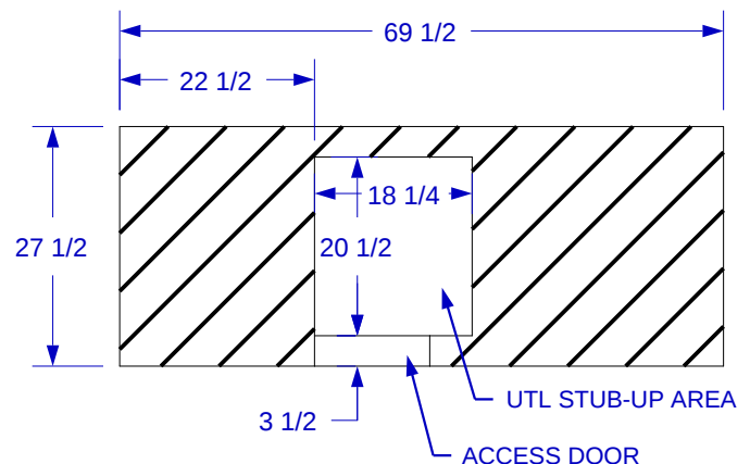
STUB-UP DIAGRAM (SEE NOTE #2)
